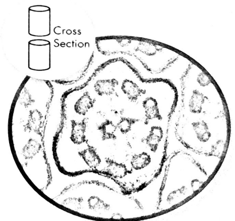
FIGURE 7-10 The “9 + 2” Pattern of Microtubules In this micrograph showing the cross section of a cilium, you can clearly see the 9 + 2 arrangement of the red microtubules. Apply Concepts What is the function of cilia?
