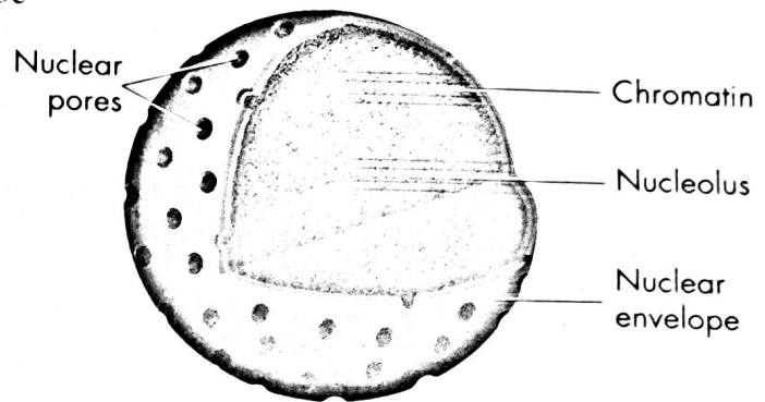
FIGURE 7-7 The Nucleus The nucleus controls most cell processes and contains DNA. The small, dense region in the nucleus is known as the nucleolus.
